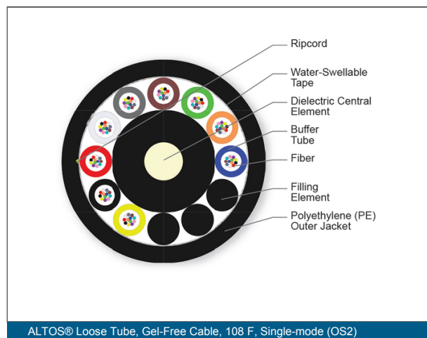
ALTOS® Loose Tube, Gel-Free Cable, 108 F, Single-mode (OS2)
