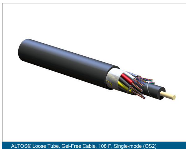
ALTOS® Loose Tube, Gel-Free Cable, 108 F, Single-mode (OS2)
